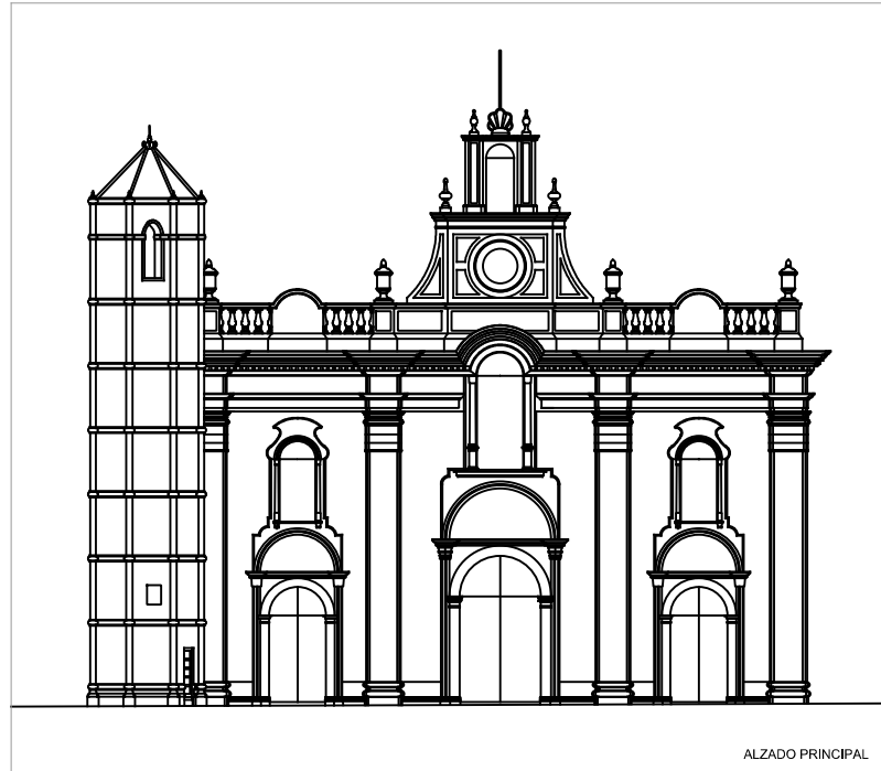
ALZADO PRINCIPAL
